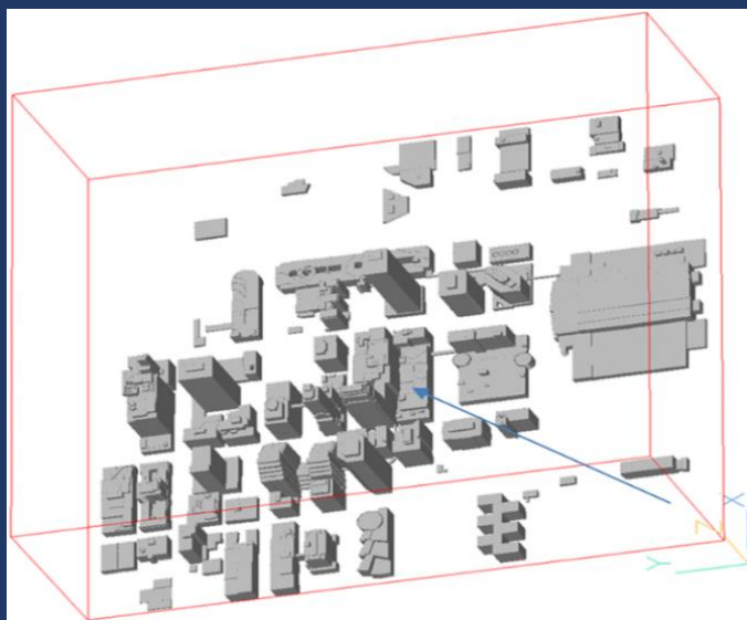
Figure 1. Solution Domain for JU2003 Experiment. The arrow indicates the main wind direction.
