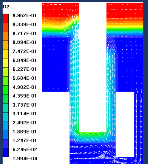
Water circulation vectors and gas phase volume fraction contours in a gas-lift evaporator.
